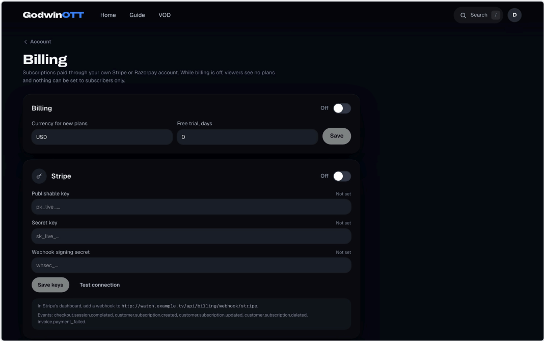
Billing is ready to switch on once provider keys are entered, and stored keys are shown only by their last four characters.
